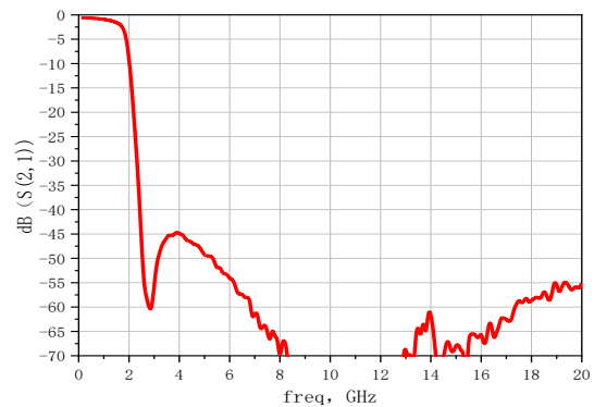
Typical Insertion Loss at T A =25
