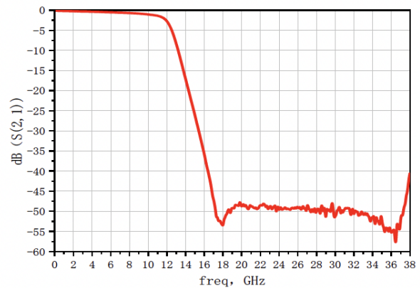
Typical Insertion Loss at T A =25
