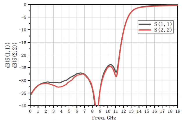
Typical Return Loss at T A =25
