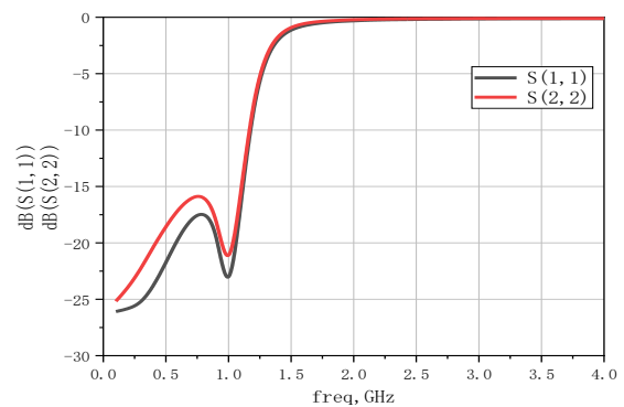
Typical Return Loss at T A =25
