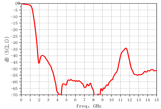
Typical widenedband Insertion Loss at T A =25°C
