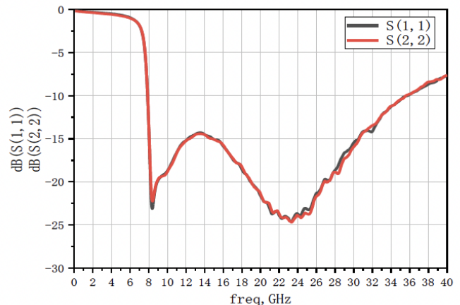
Typical Return Loss at T A =25
